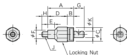
QLTL-RA (Plug-In-Handle Adaptors)
